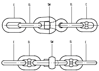
SWIVEL PIECE=SP
