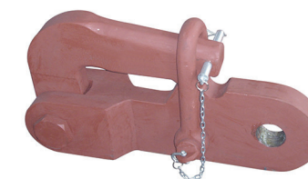
Marine Quick Release Pelican Hook
