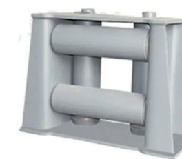
FAIRLEAD ROLLER
