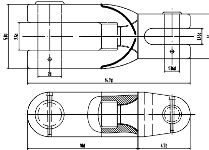
ANCHOR SWIVEL SHACKLE (a)
