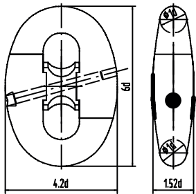
KENTER SHACKLE=KS
