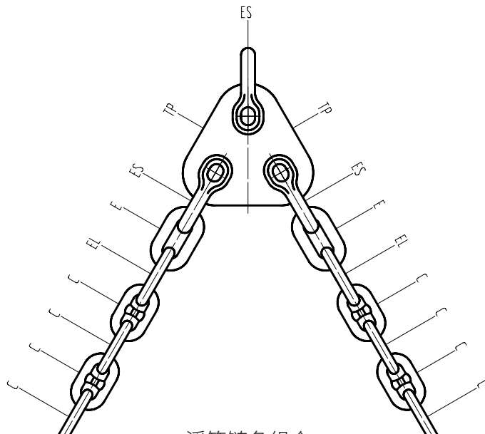
浮筒链条组合 BUOY CHAIN SET
