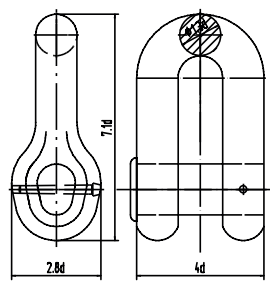
JOINING SHACKLE=JS
