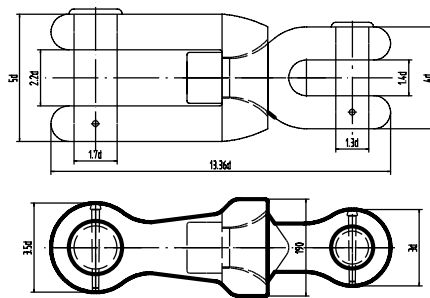
ANCHOR SWIVEL SHACKLE (b)
