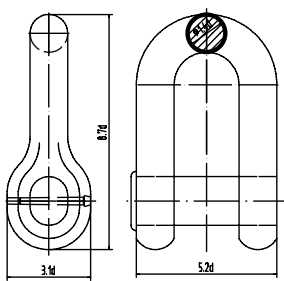
END SHACKLE=ES
