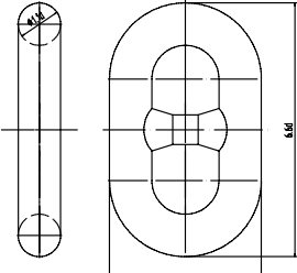
ENLARGED LINK=EL
